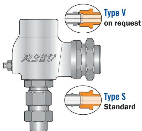
4) Butt-Welding fittings inlet & outlet (3 pieces union couplings)
