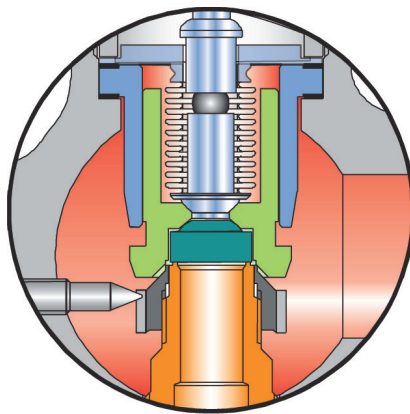
2) Balanced Bellows (D & F Orifices)
