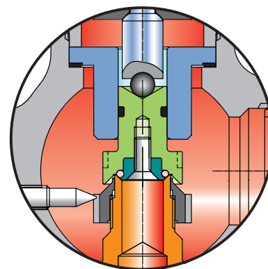
6b) Balanced Soft seat
