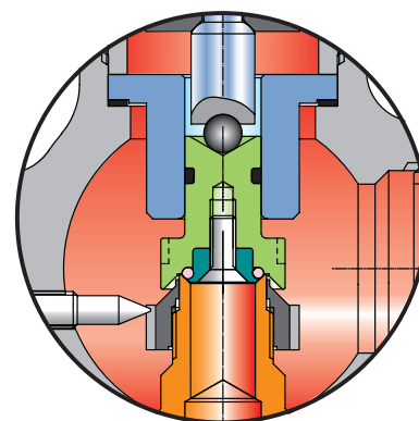
6a) Conventional Soft seat
